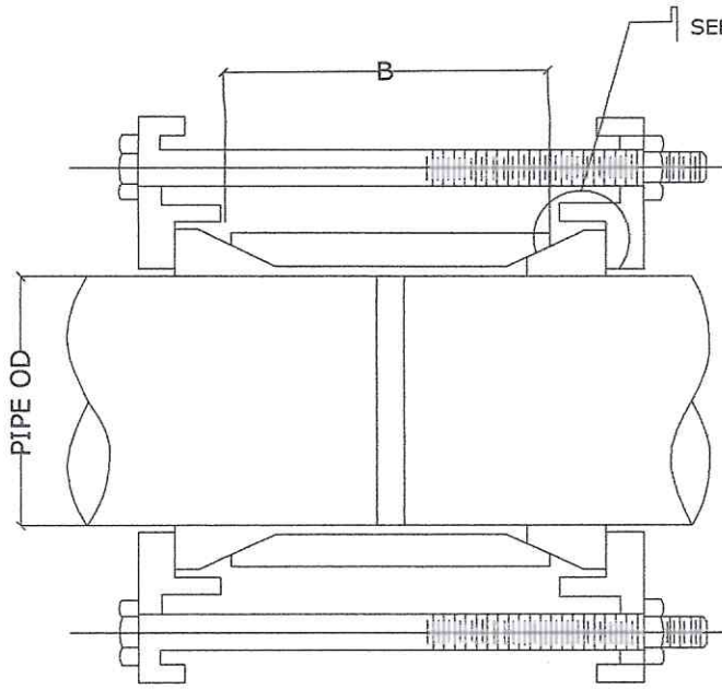
C.I SLEEVE TYPE COUPLING FOR GIP
